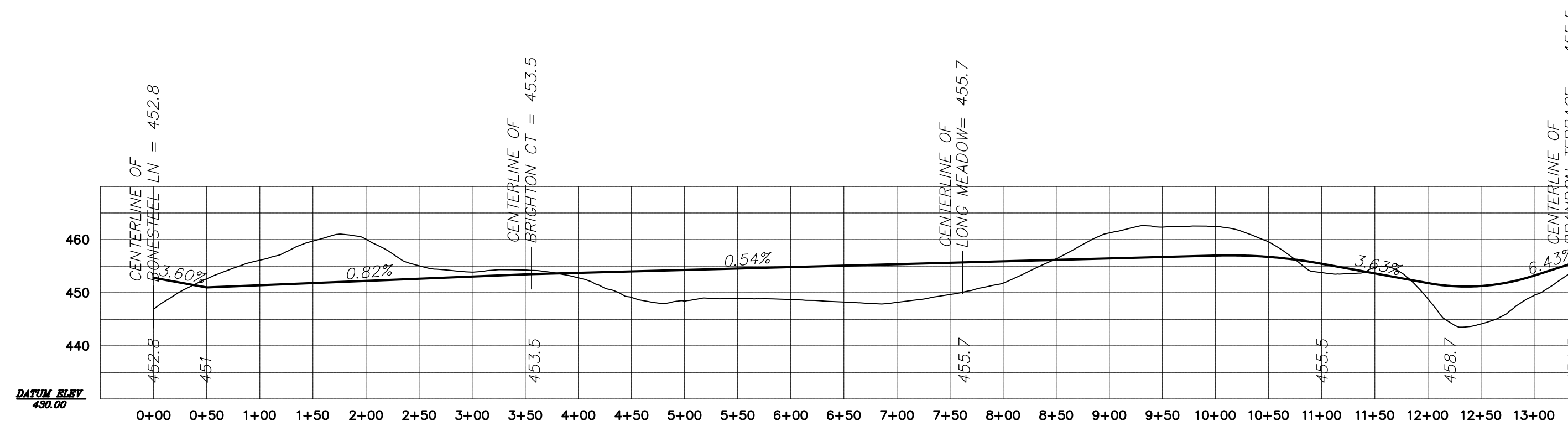
BRANDON TERRACE SCALE: H 1"=100', V 1"=20'
